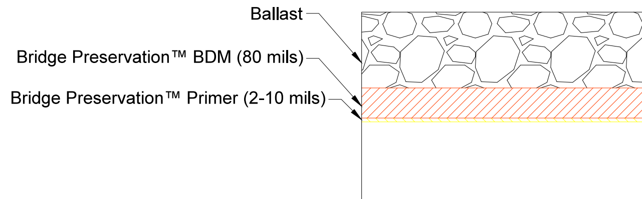
Detail A
